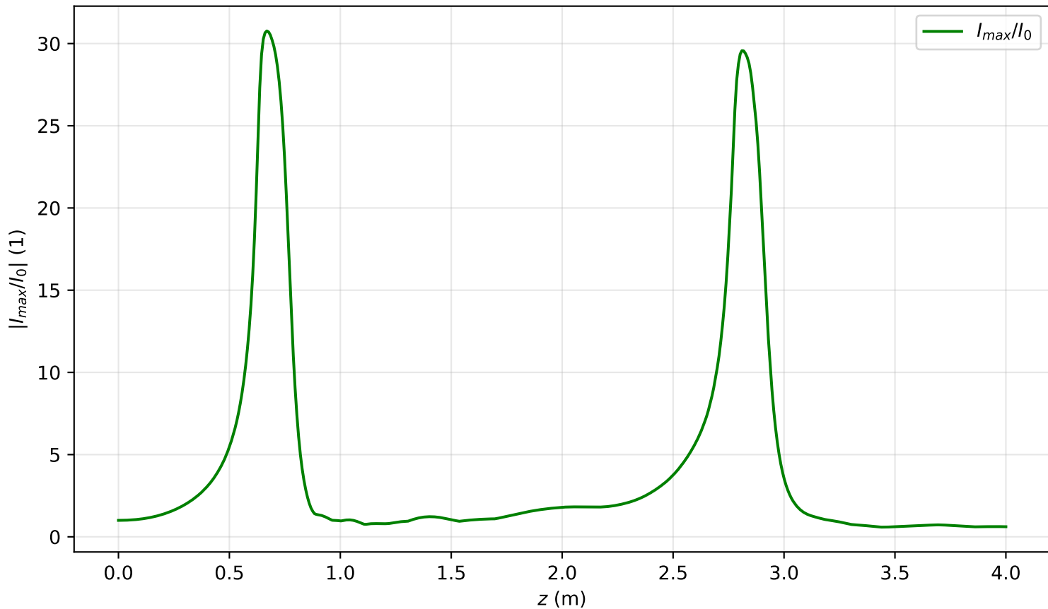
I_{max}(x = 0, y = 0, z)/I_0 , Pin=7.0P_{cr} , artificial time
